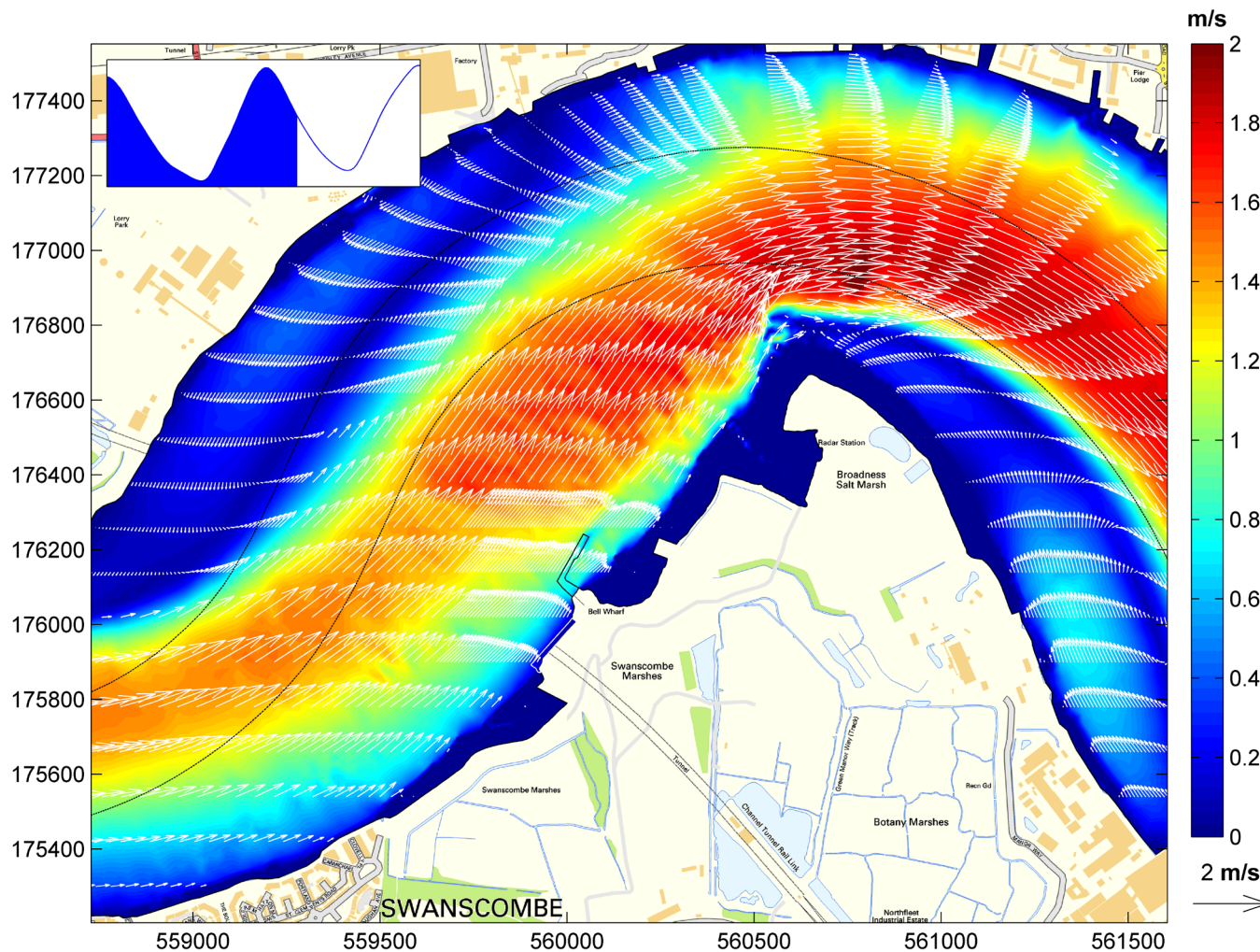
Figure 17.18: Kent Project Site Baseline Hydrodynamic showing current magnitude at time peak ebb tide.
